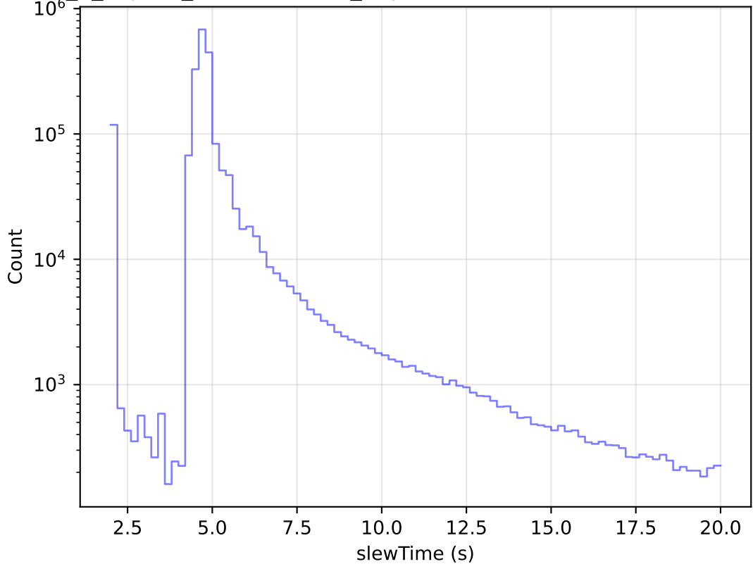
internal_u_expt45_nscale1.5v3.4_10yrs All visits: Zoom Slew Time Histogram
