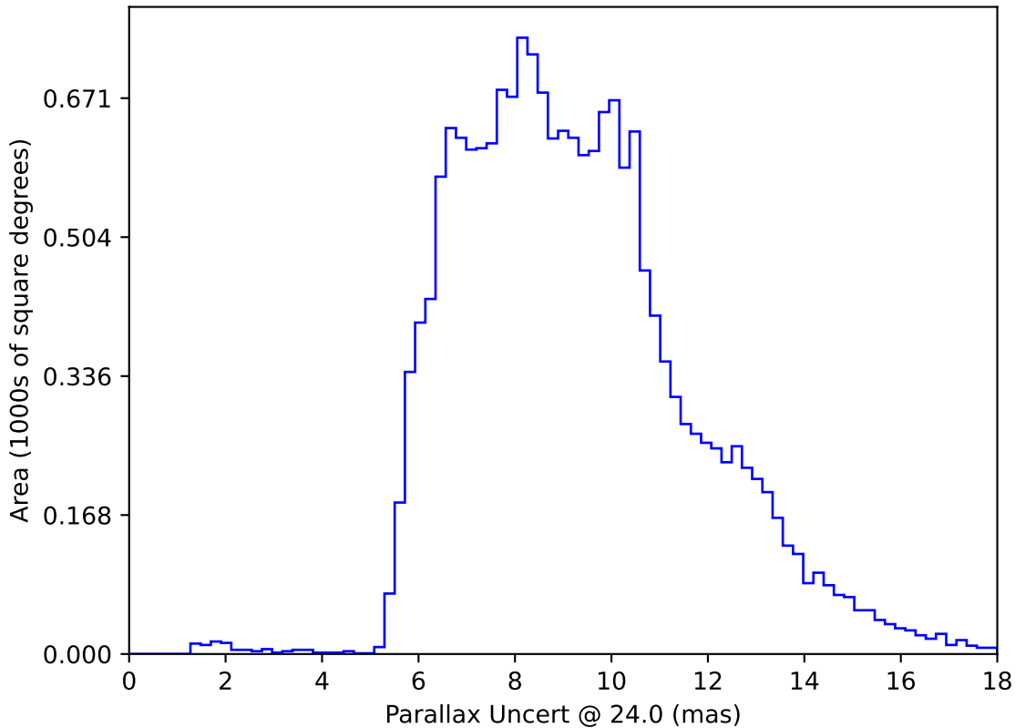
internal_u_expt45_nscale1.5v3.4_10yrs WFD: Parallax Uncert @ 24.0
