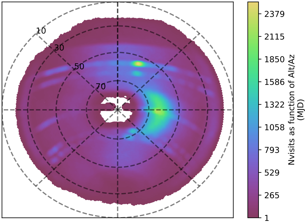
internal_u_expt45_nscale1.5v3.4_10yrs z band: Nvisits as function of Alt/Az
