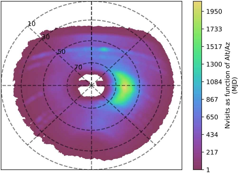
internal_u_expt45_nscale1.5v3.4_10yrs y band: Nvisits as function of Alt/Az
