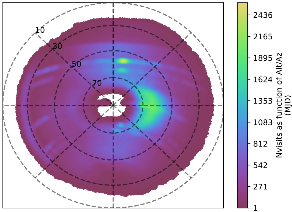
internal_u_expt45_nscale1.5v3.4_10yrs r band: Nvisits as function of Alt/Az
