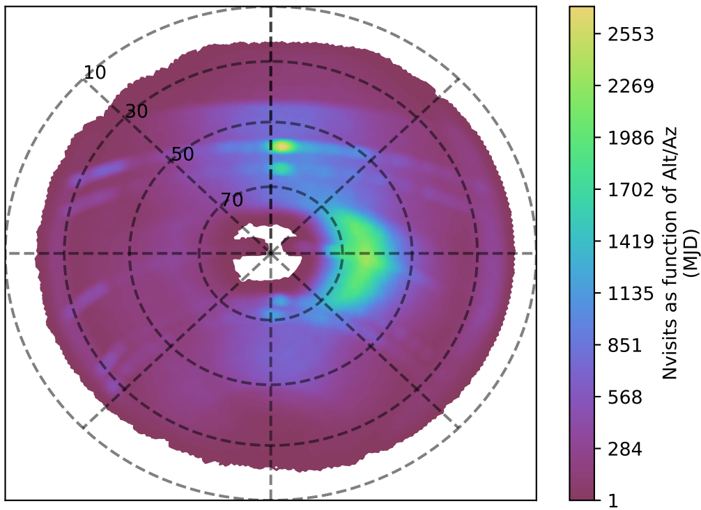
internal_u_expt45_nscale1.5v3.4_10yrs i band: Nvisits as function of Alt/Az
