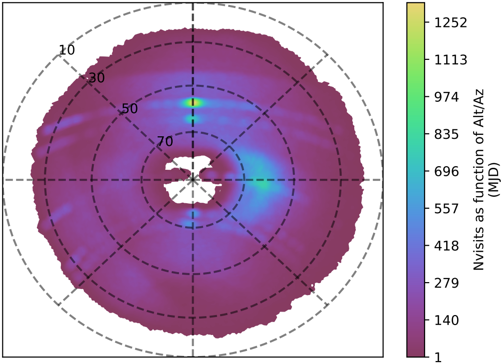
internal_u_expt45_nscale1.5v3.4_10yrs g band: Nvisits as function of Alt/Az
