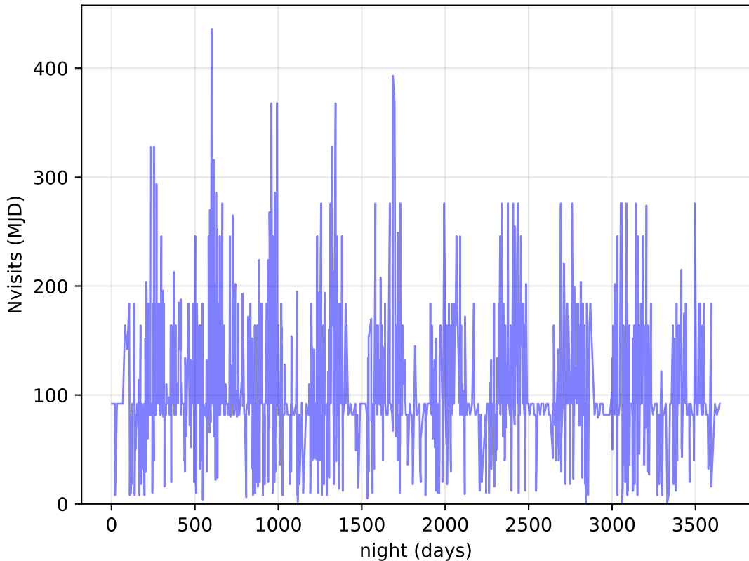
internal_u_expt45_nscale1.5v3.4_10yrs DDF: Nvisits
