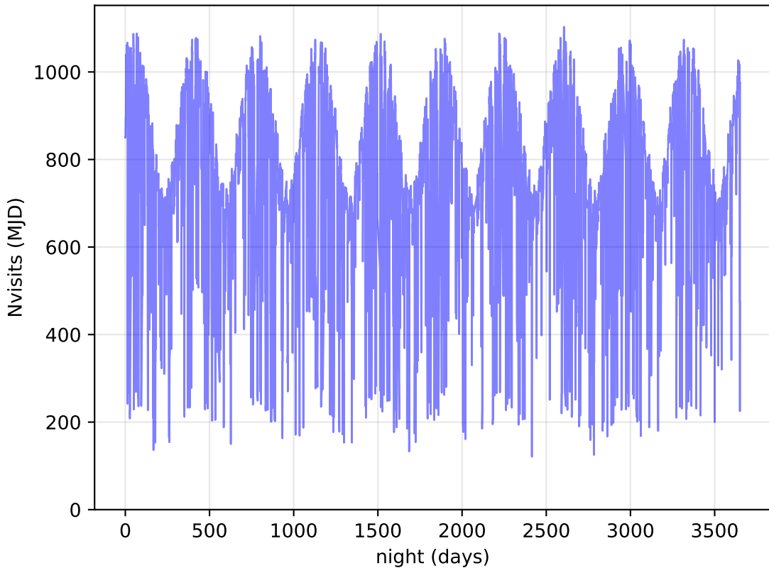
internal_u_expt45_nscale1.5v3.4_10yrs All visits: Nvisits
