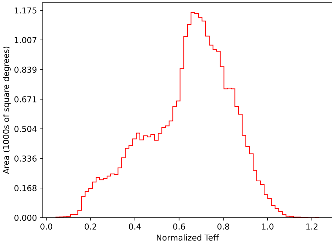
internal_u_expt45_nscale1.5v3.4_10yrs All sky i band: Normalized Teff
