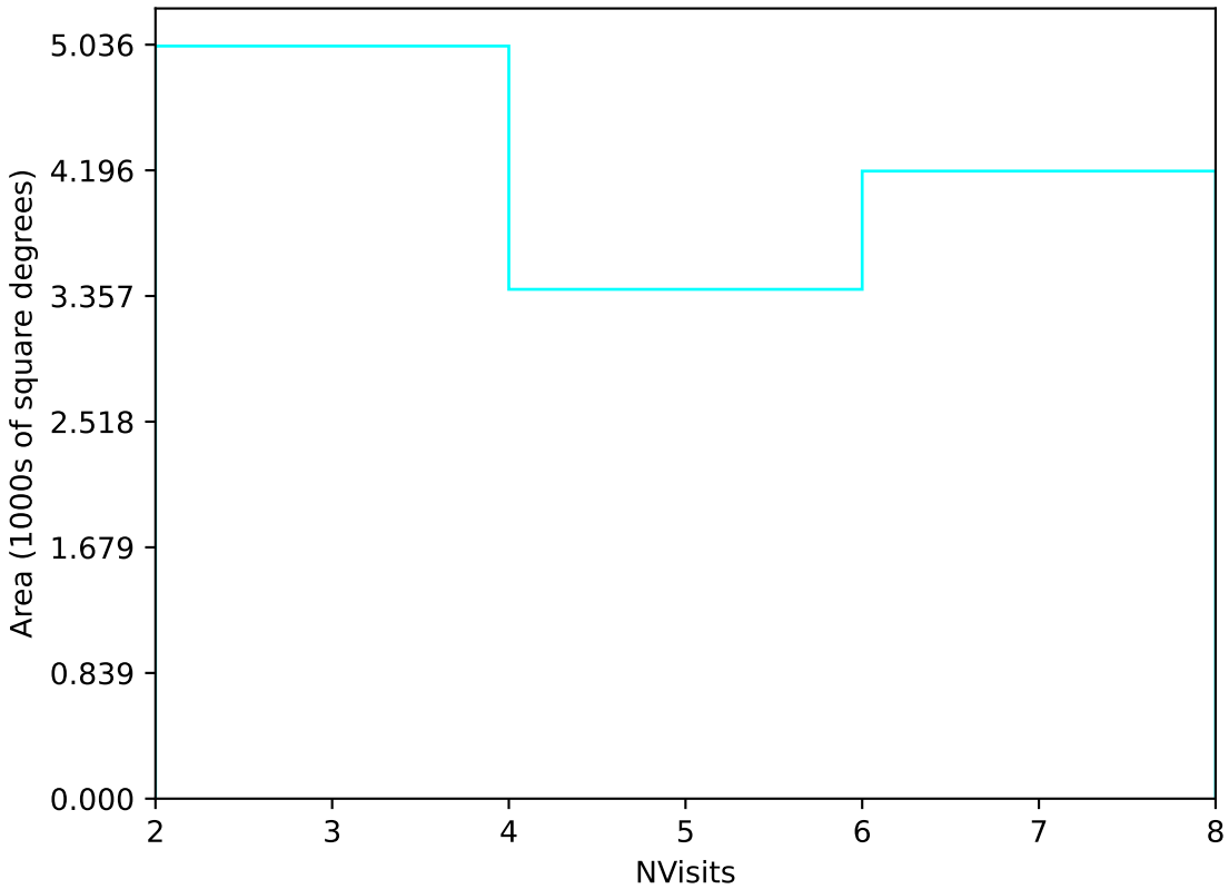
internal_u_expt45_nscale1.5v3.4_10yrs Yr 3-4 u band: NVisits
