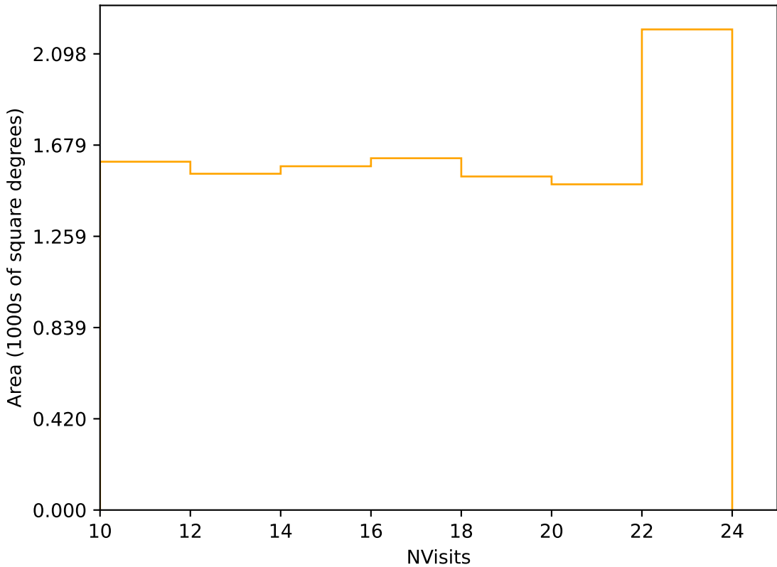
internal_u_expt45_nscale1.5v3.4_10yrs Yr 3-4 r band: NVisits
