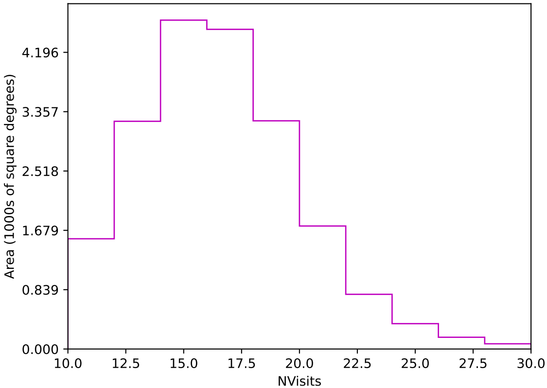
internal_u_expt45_nscale1.5v3.4_10yrs Yr 1 z band: NVisits
