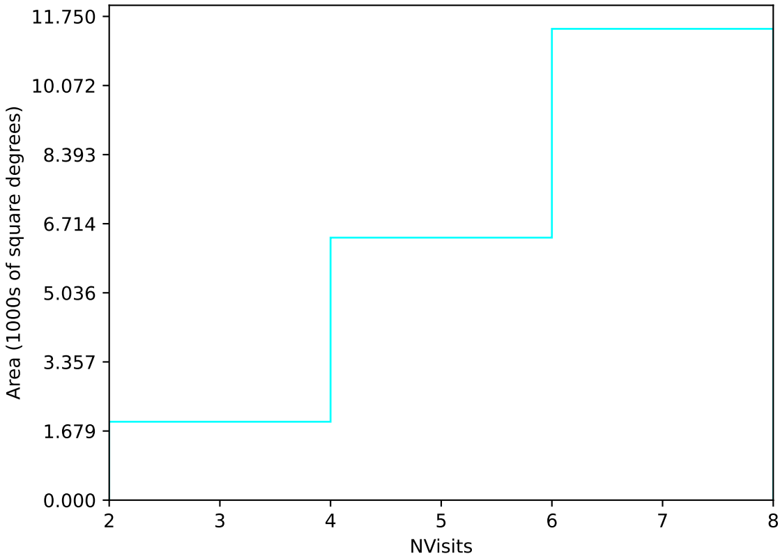
internal_u_expt45_nscale1.5v3.4_10yrs Yr 1 u band: NVisits
