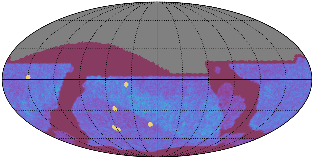
internal_u_expt45_nscale1.5v3.4_10yrs All sky z band: NVisits
