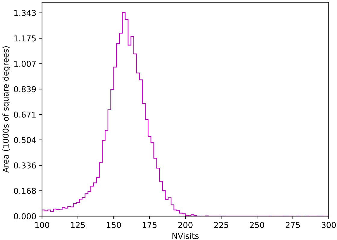
internal_u_expt45_nscale1.5v3.4_10yrs All sky z band: NVisits
