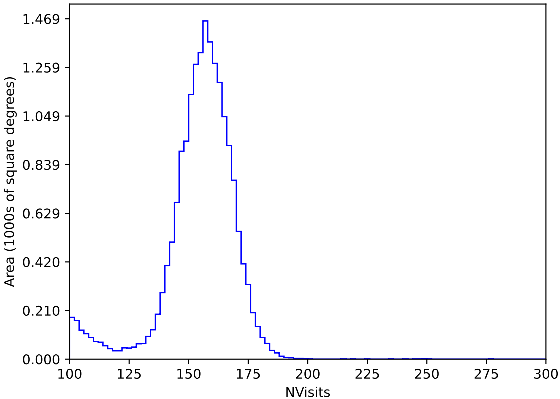
internal_u_expt45_nscale1.5v3.4_10yrs All sky y band: NVisits
