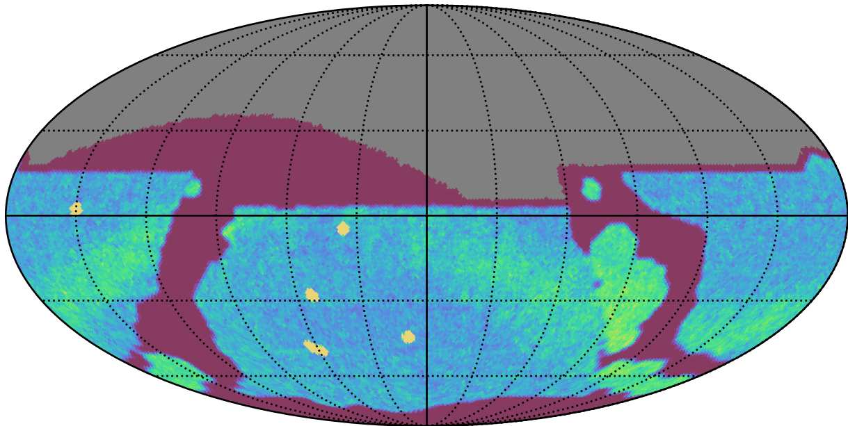
internal_u_expt45_nscale1.5v3.4_10yrs All sky r band: NVisits
