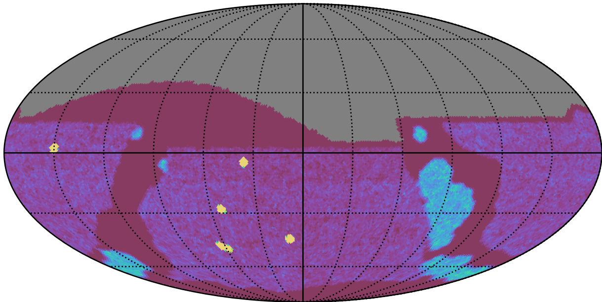
internal_u_expt45_nscale1.5v3.4_10yrs All sky g band: NVisits
