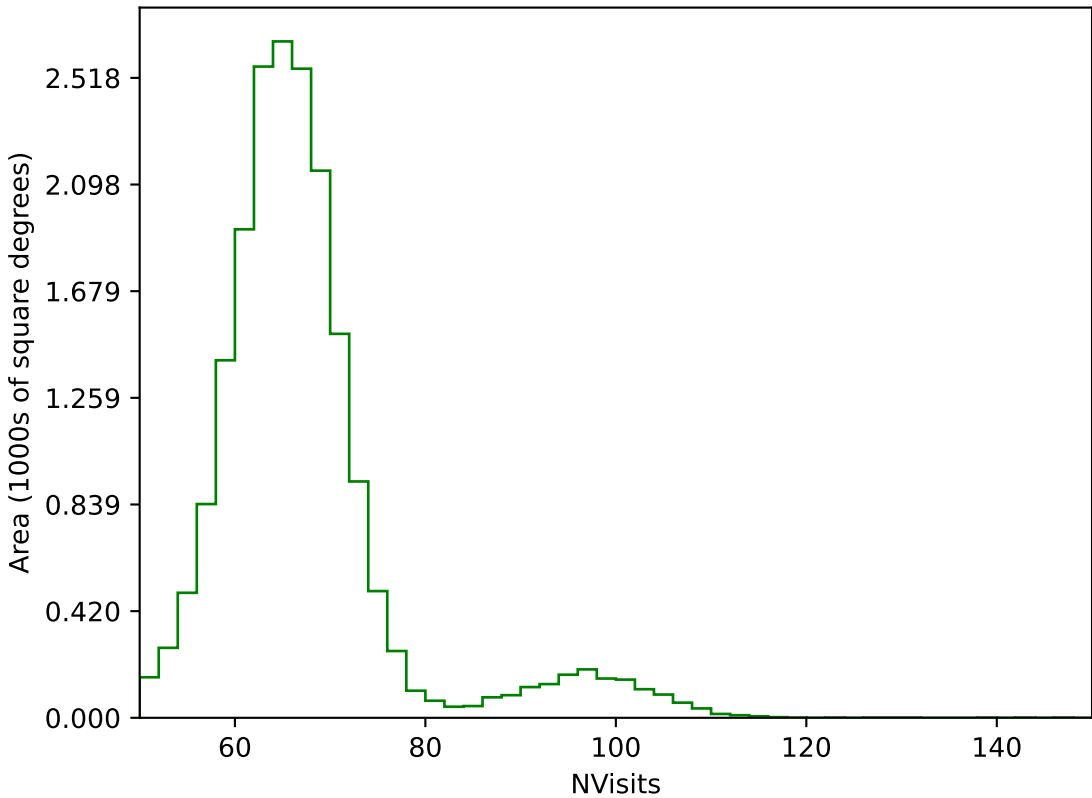
internal_u_expt45_nscale1.5v3.4_10yrs All sky g band: NVisits
