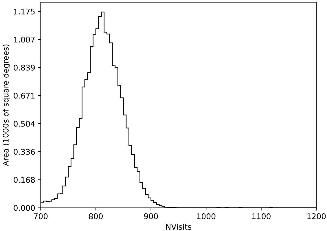
internal_u_expt45_nscale1.5v3.4_10yrs All sky all bands: NVisits
