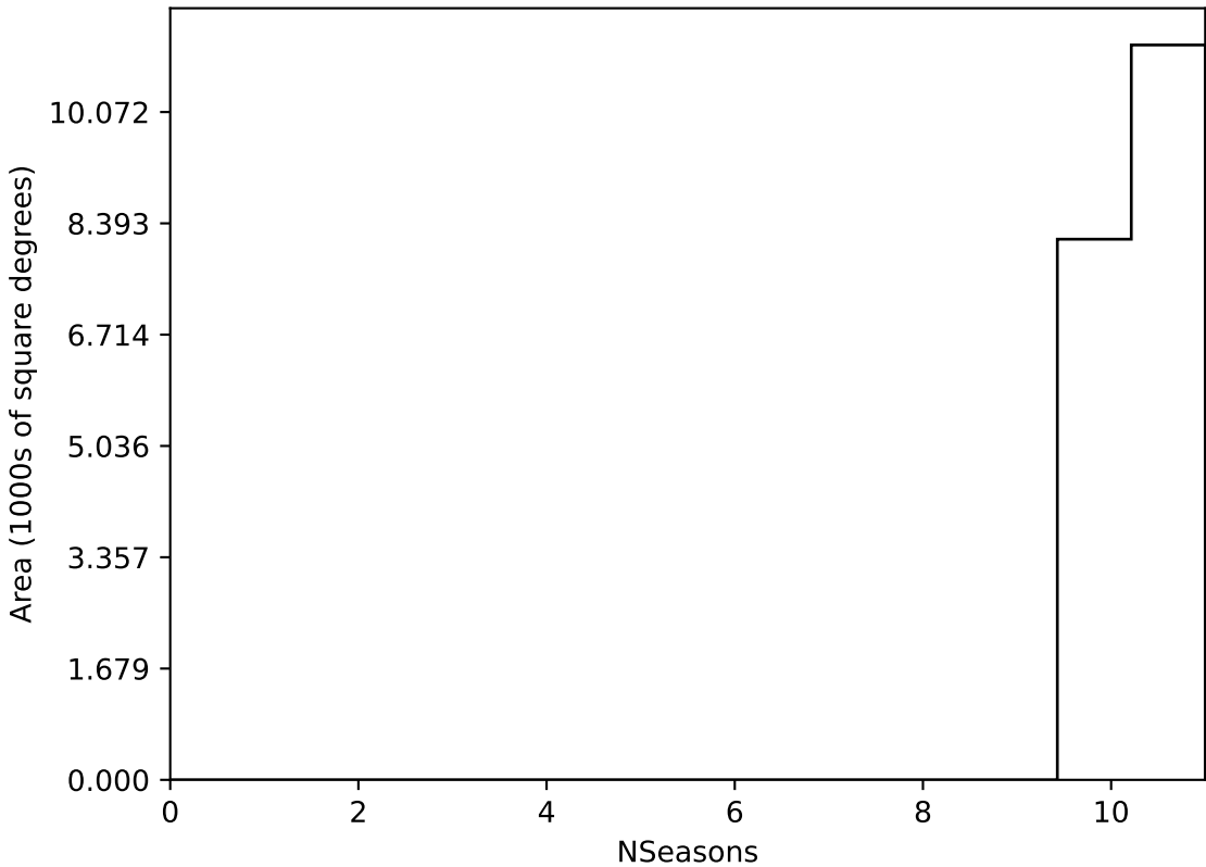
internal_u_expt45_nscale1.5v3.4_10yrs WFD all bands: NSeasons
