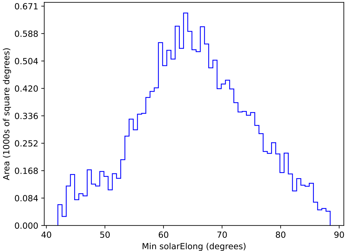
internal_u_expt45_nscale1.5v3.4_10yrs WFD y band: Min solarElong
