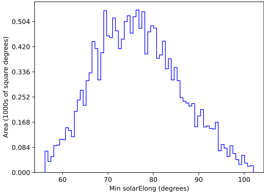
internal_u_expt45_nscale1.5v3.4_10yrs WFD g band: Min solarElong
