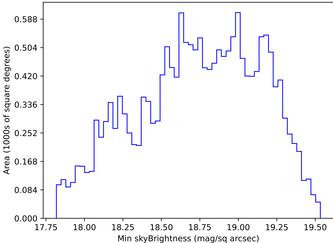
internal_u_expt45_nscale1.5v3.4_10yrs WFD r band: Min skyBrightness
