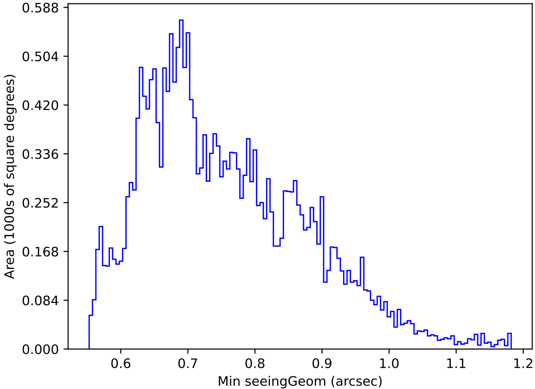
internal_u_expt45_nscale1.5v3.4_10yrs Yr 1 u band: Min seeingGeom
