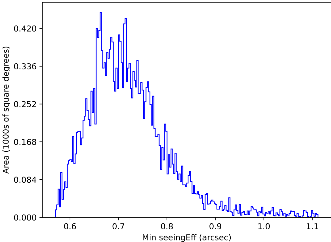
internal_u_expt45_nscale1.5v3.4_10yrs Yr 1 y band: Min seeingEff
