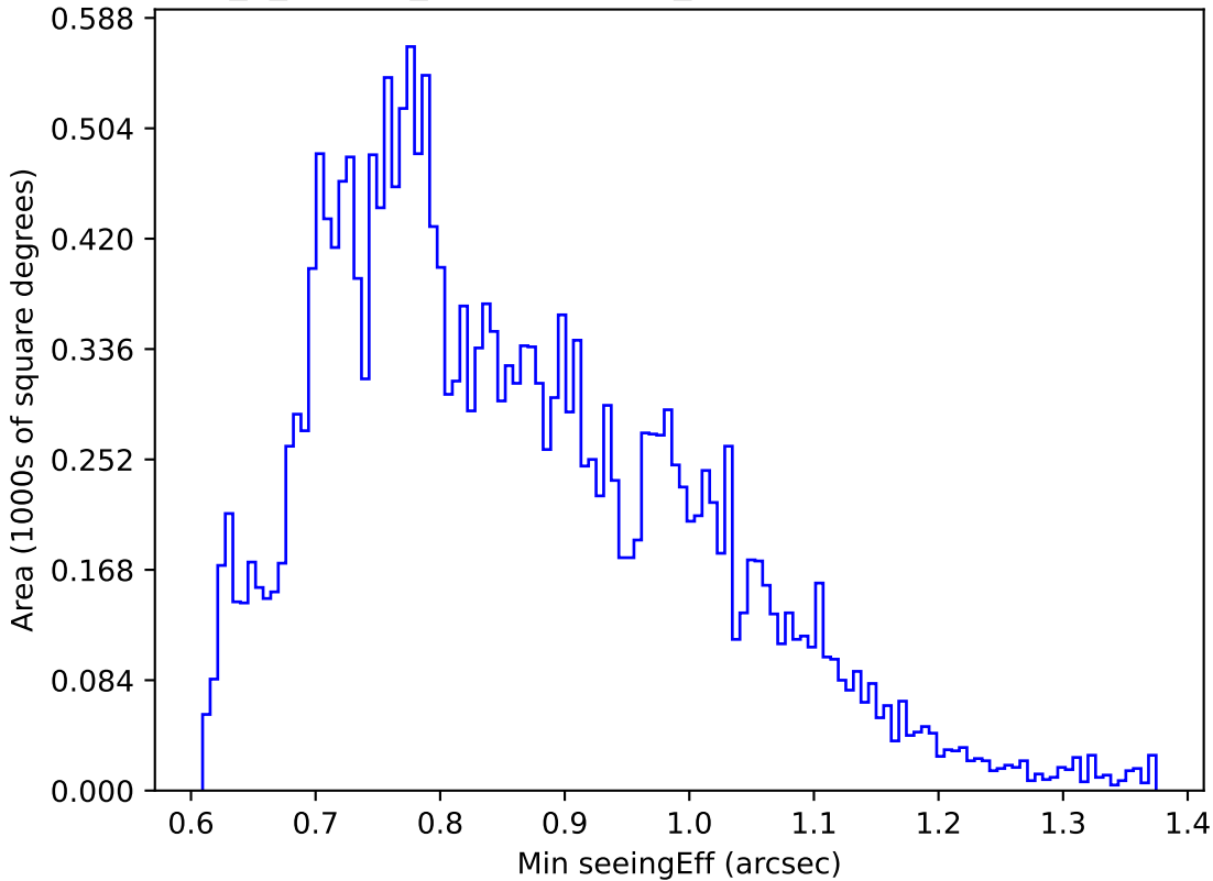
internal_u_expt45_nscale1.5v3.4_10yrs Yr 1 u band: Min seeingEff
