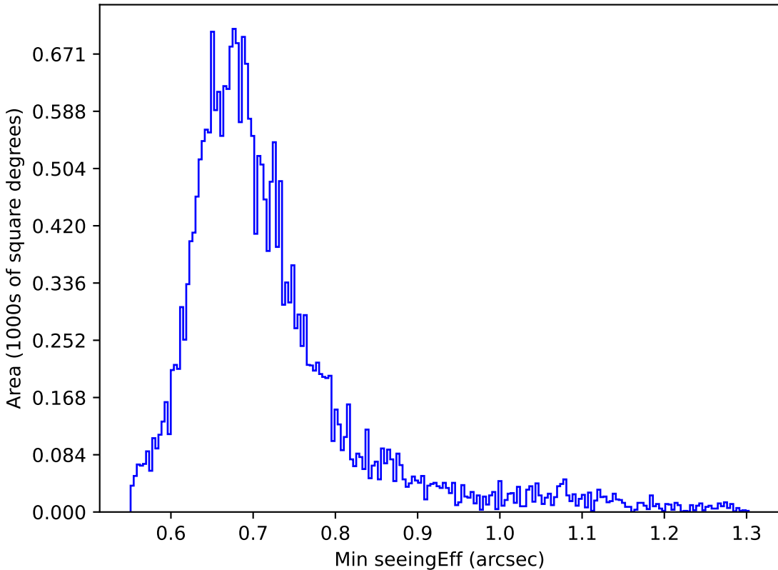
internal_u_expt45_nscale1.5v3.4_10yrs Yr 1 r band: Min seeingEff
