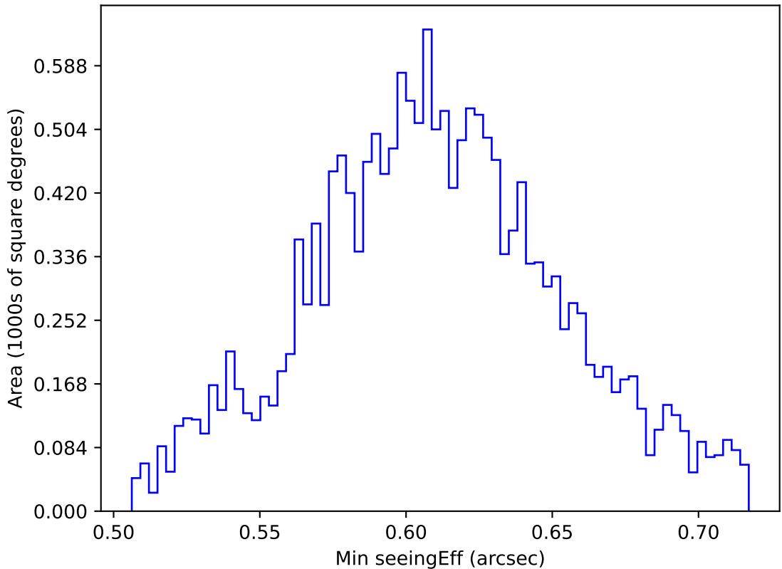
internal_u_expt45_nscale1.5v3.4_10yrs WFD z band: Min seeingEff
