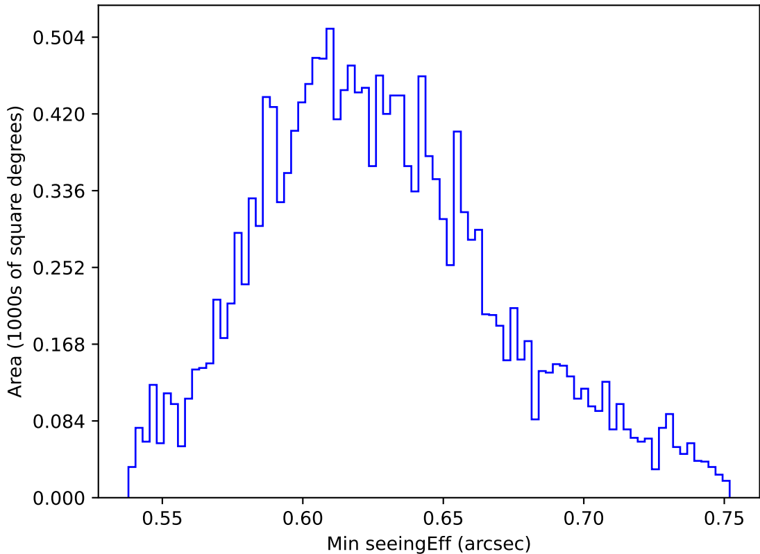
internal_u_expt45_nscale1.5v3.4_10yrs WFD y band: Min seeingEff
