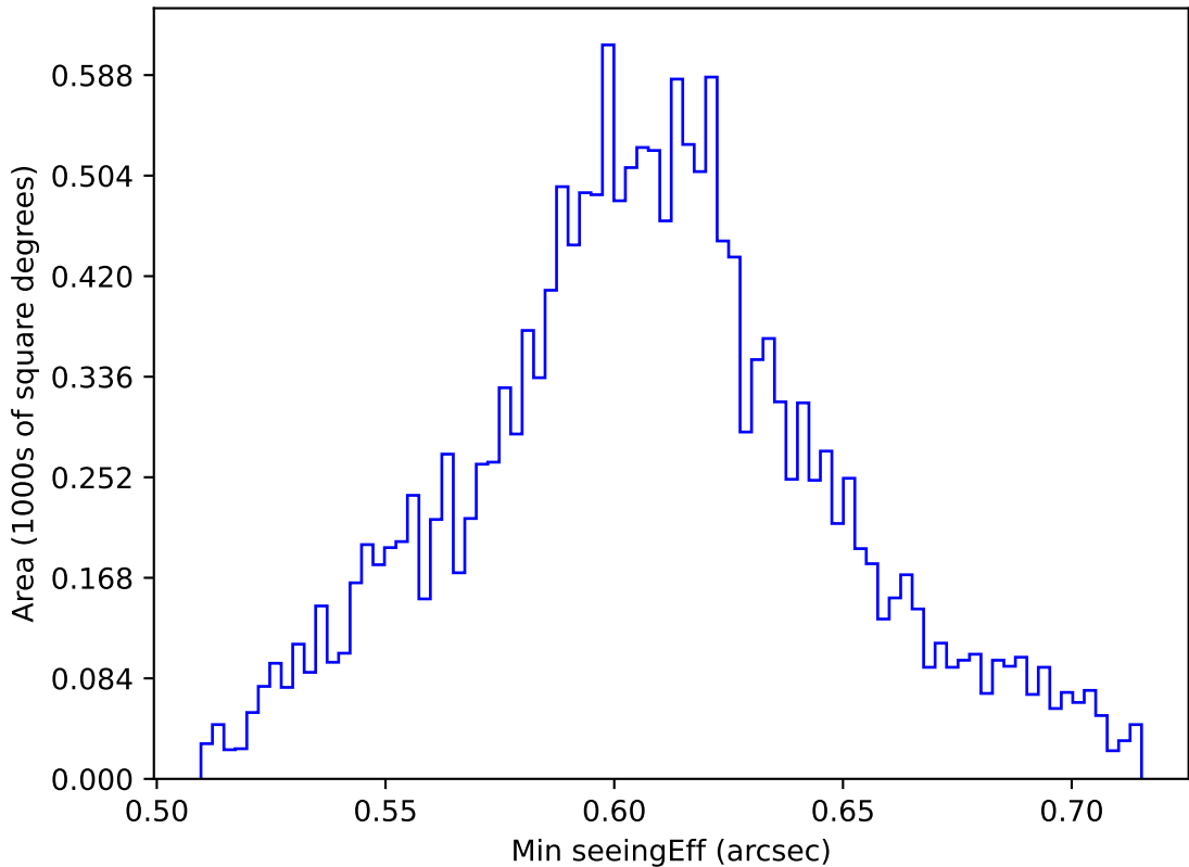
internal_u_expt45_nscale1.5v3.4_10yrs WFD i band: Min seeingEff
