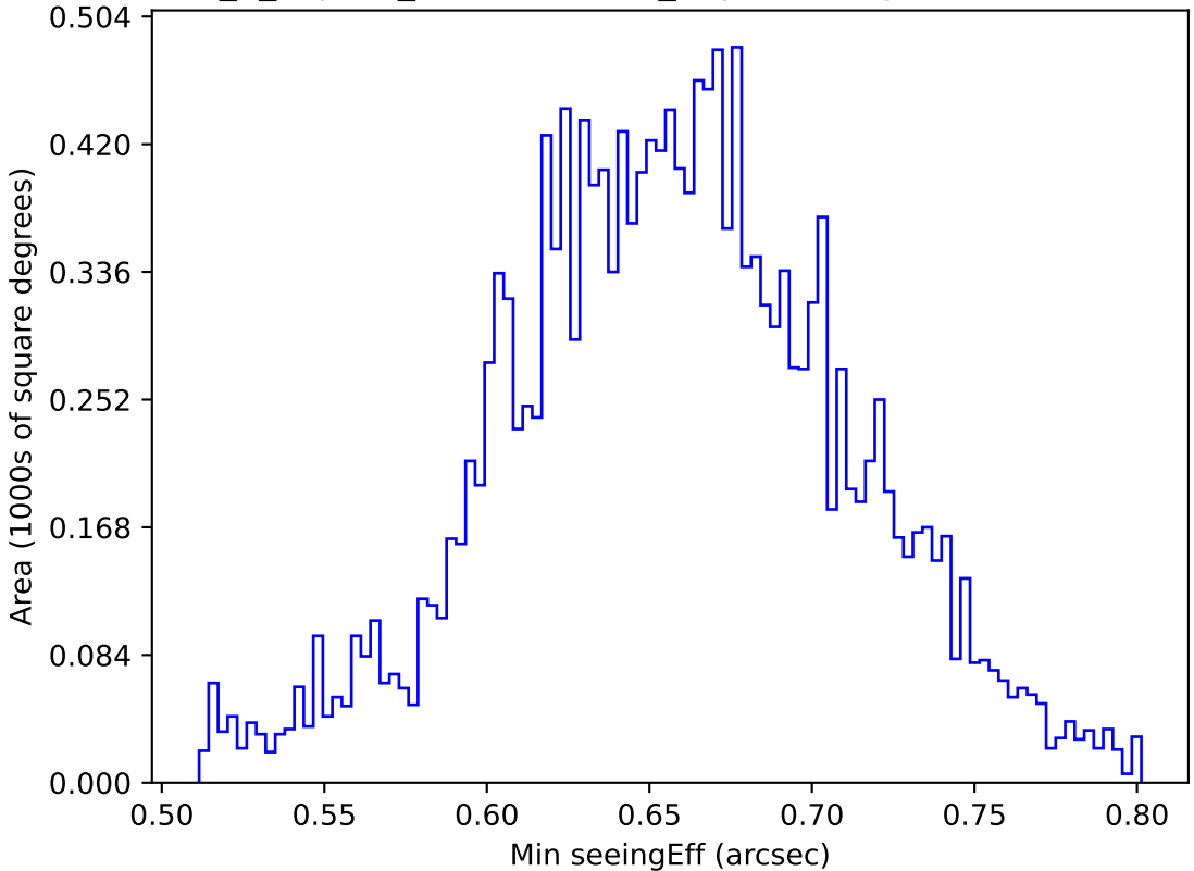
internal_u_expt45_nscale1.5v3.4_10yrs WFD g band: Min seeingEff
