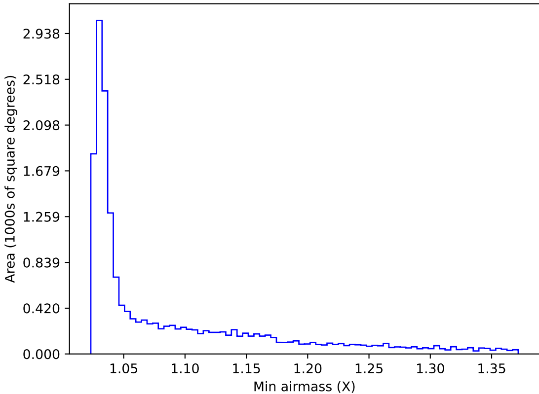
internal_u_expt45_nscale1.5v3.4_10yrs WFD y band: Min airmass
