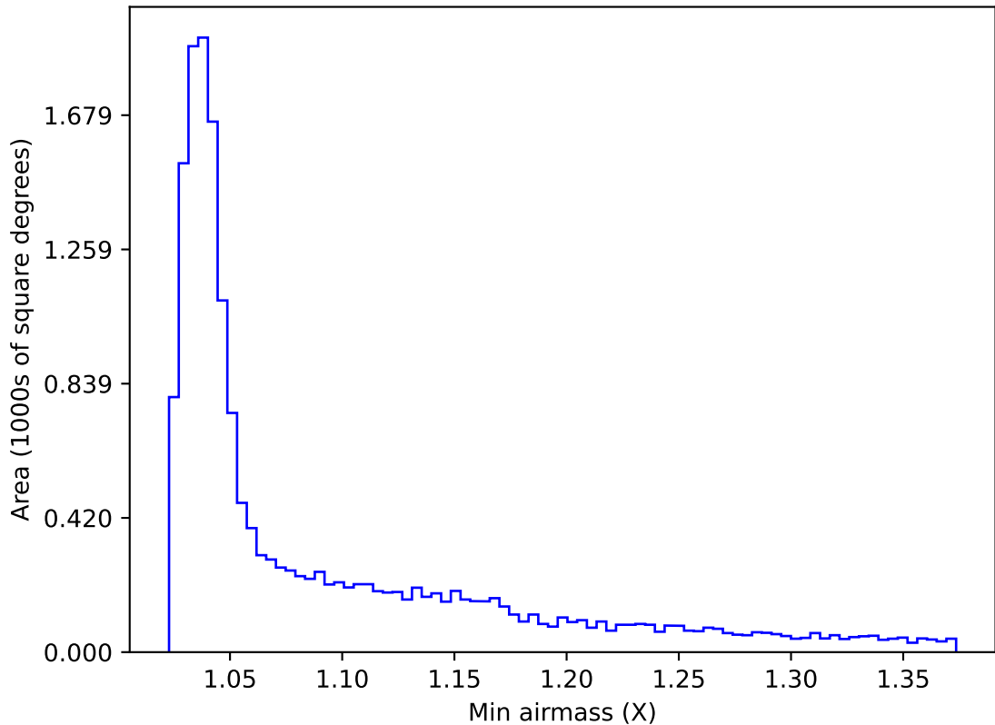
internal_u_expt45_nscale1.5v3.4_10yrs WFD u band: Min airmass
