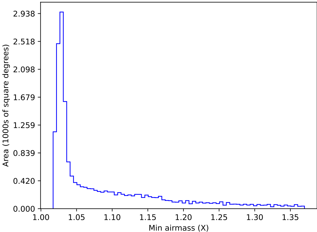
internal_u_expt45_nscale1.5v3.4_10yrs WFD r band: Min airmass
