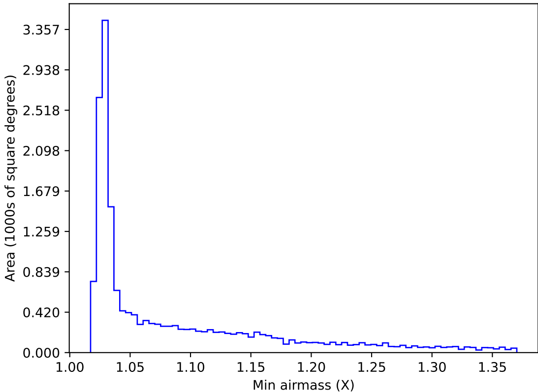
internal_u_expt45_nscale1.5v3.4_10yrs WFD i band: Min airmass
