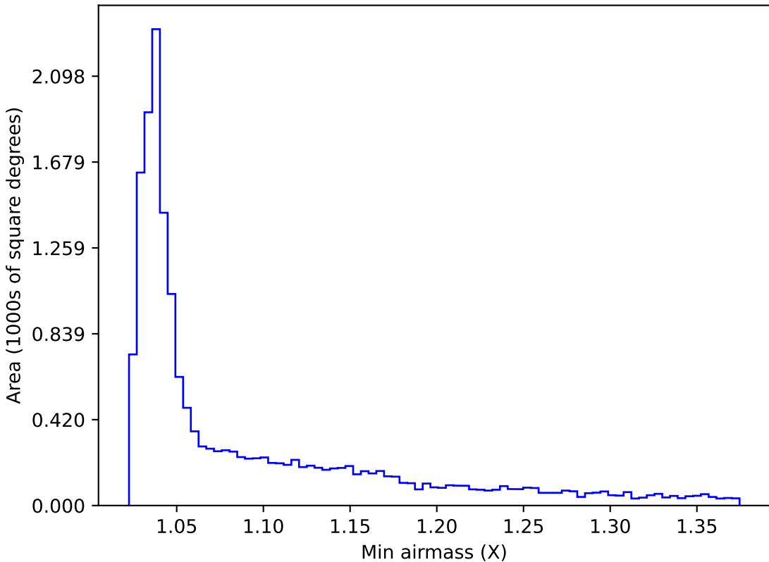
internal_u_expt45_nscale1.5v3.4_10yrs WFD g band: Min airmass
