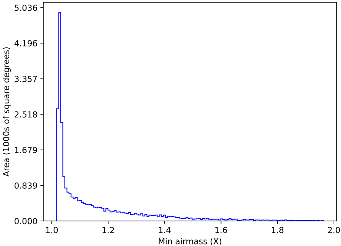
internal_u_expt45_nscale1.5v3.4_10yrs All sky r band: Min airmass
