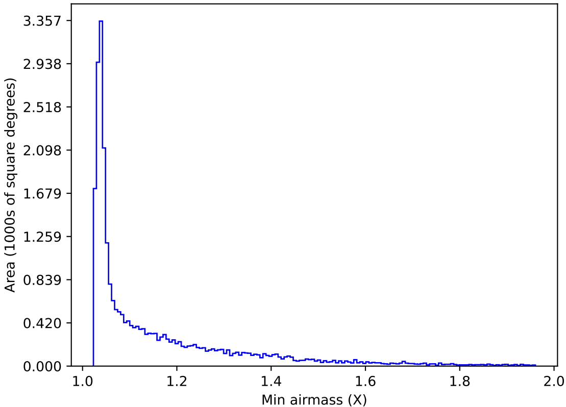
internal_u_expt45_nscale1.5v3.4_10yrs All sky g band: Min airmass
