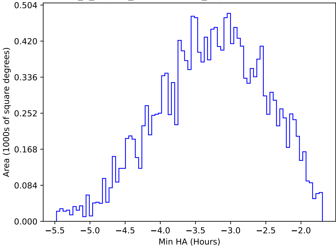
internal_u_expt45_nscale1.5v3.4_10yrs WFD u band: Min HA
