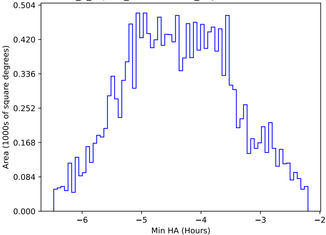
internal_u_expt45_nscale1.5v3.4_10yrs WFD i band: Min HA
