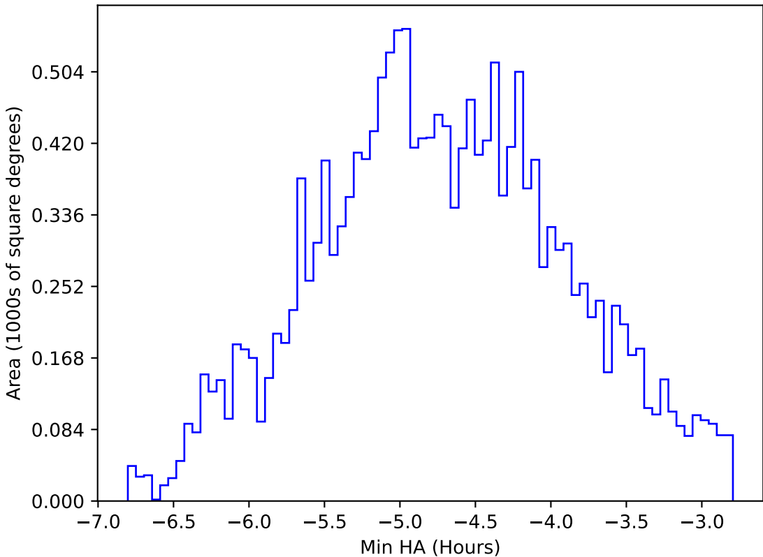
internal_u_expt45_nscale1.5v3.4_10yrs WFD all bands: Min HA
