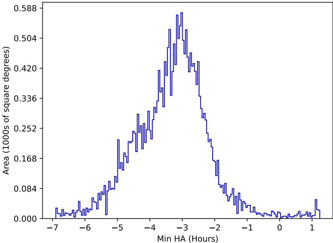
internal_u_expt45_nscale1.5v3.4_10yrs All sky y band: Min HA
