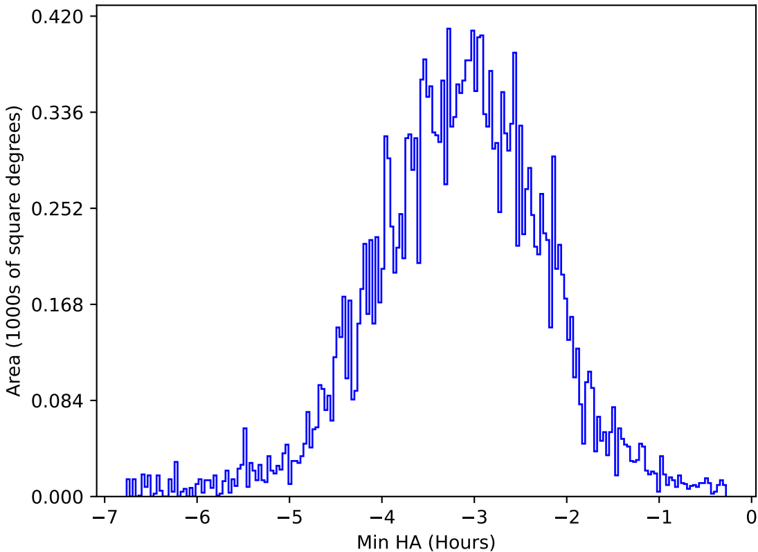
internal_u_expt45_nscale1.5v3.4_10yrs All sky u band: Min HA
