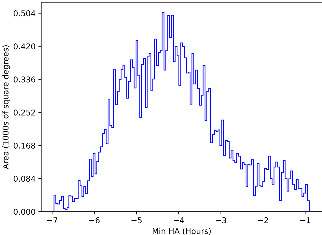
internal_u_expt45_nscale1.5v3.4_10yrs All sky r band: Min HA
