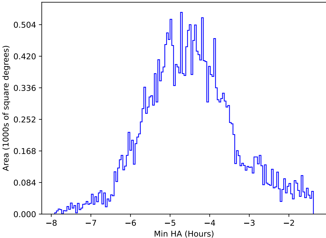
internal_u_expt45_nscale1.5v3.4_10yrs All sky all bands: Min HA
