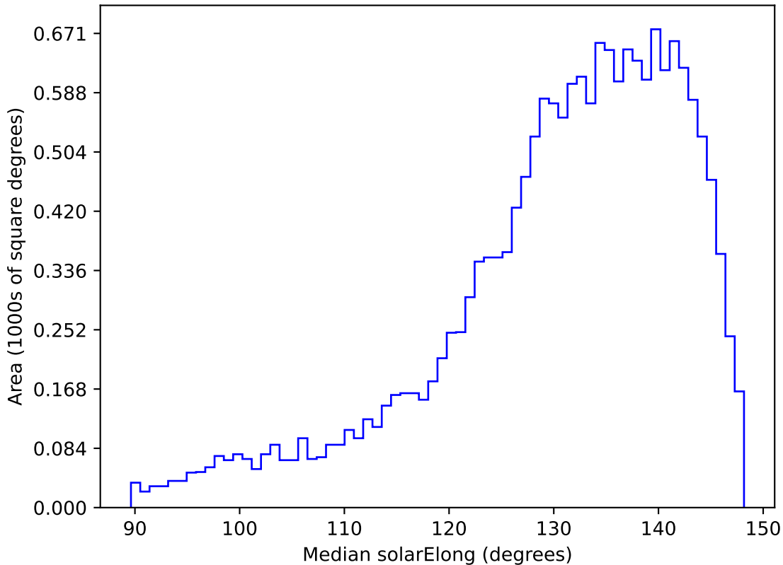
internal_u_expt45_nscale1.5v3.4_10yrs WFD r band: Median solarElong
