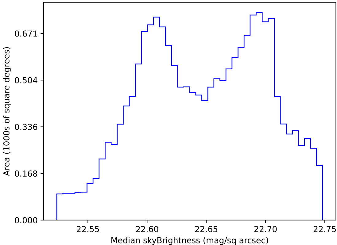
internal_u_expt45_nscale1.5v3.4_10yrs WFD u band: Median skyBrightness
