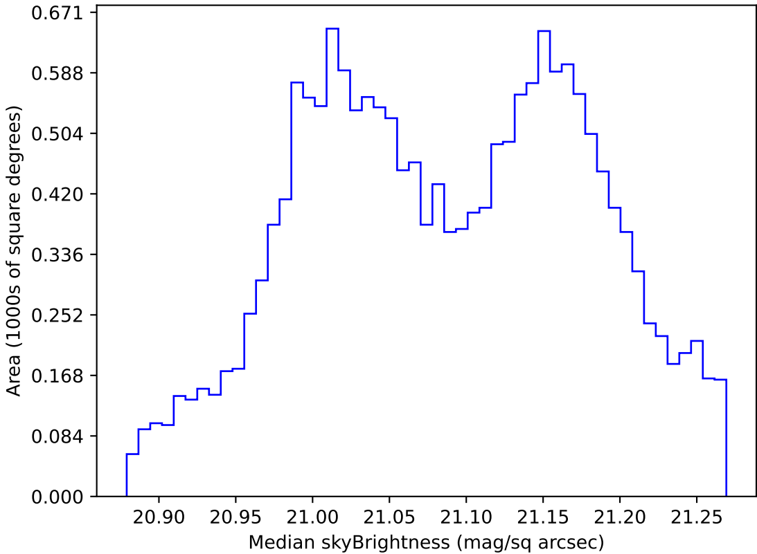
internal_u_expt45_nscale1.5v3.4_10yrs WFD r band: Median skyBrightness
